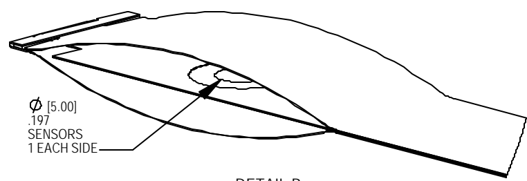
DETAIL B SCALE 2 : 1
